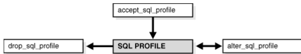
Figure 12-4 SQL Profiles APIs
