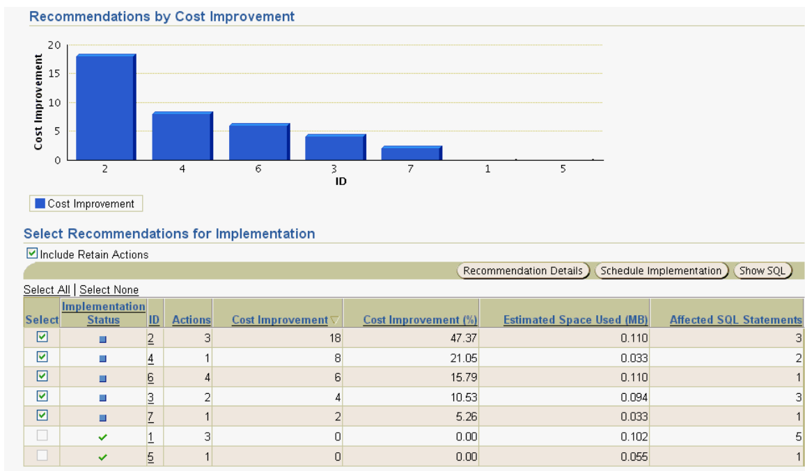
Figure 17–10 SQL Access Advisor: Recommendation Details
