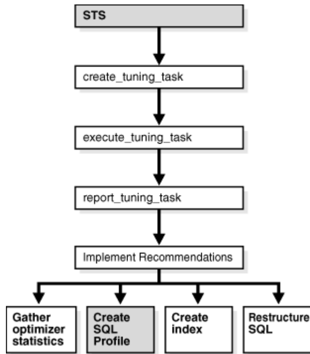
Figure 12-2 SQL Tuning Advisor APIs
