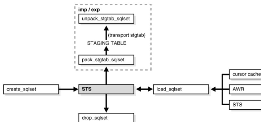
Figure 12-3 SQL Tuning Sets APIs
