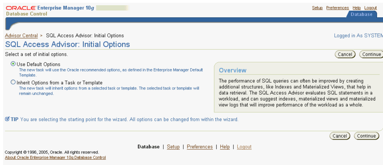
Figure 17–3 SQL Access Advisor: Selecting the Initial Options
