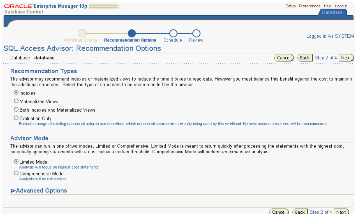
Figure 17–5 SQL Access Advisor: Choosing the Recommendation Options
