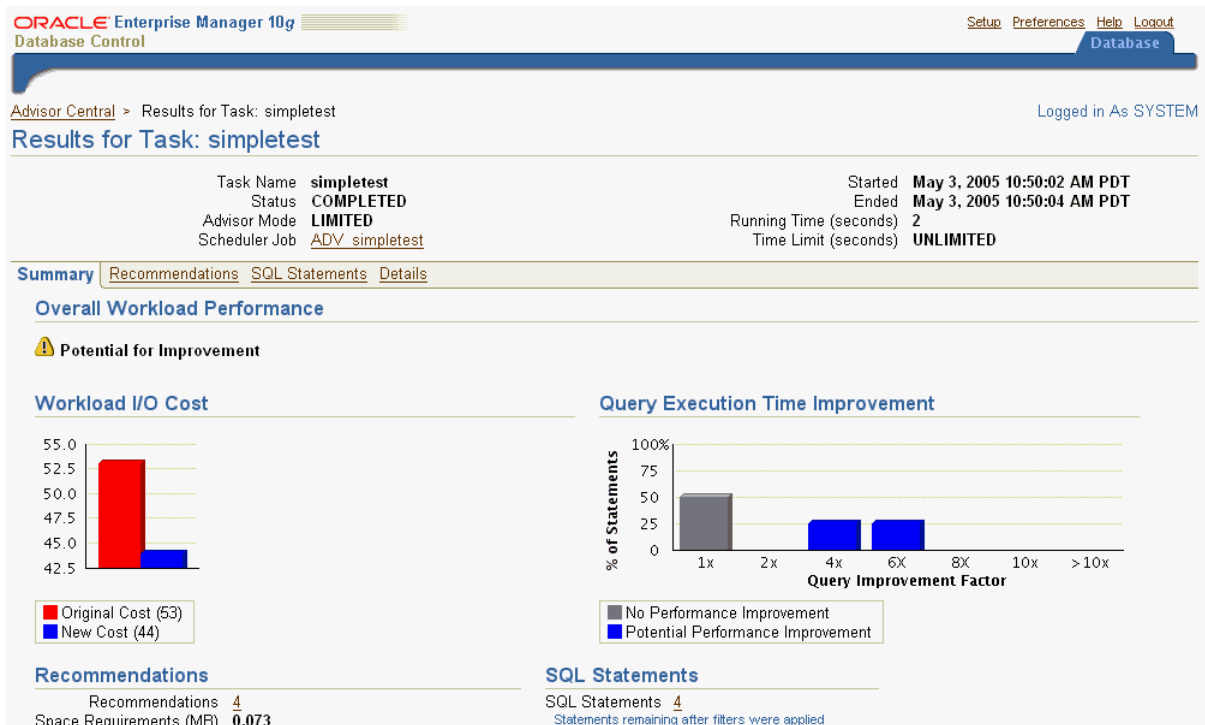
Figure 17–9 SQL Access Advisor: Overview of the Recommendations
