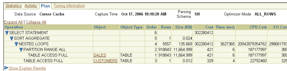
Figure 9–7 Viewing SQL Execution Plan
