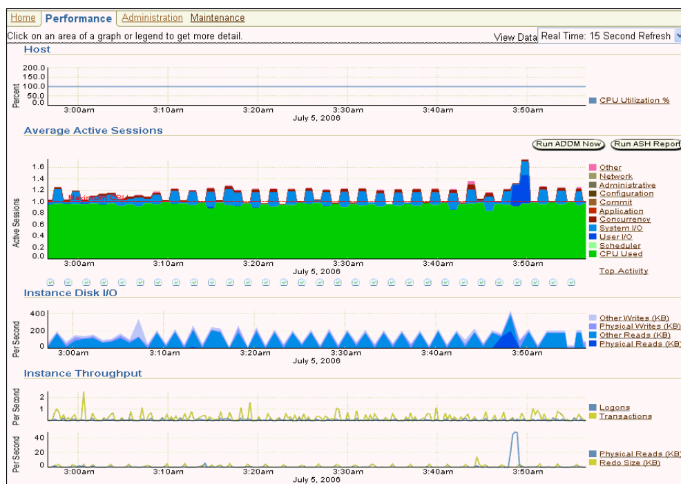
Figure 4-1 Database Performance Page
