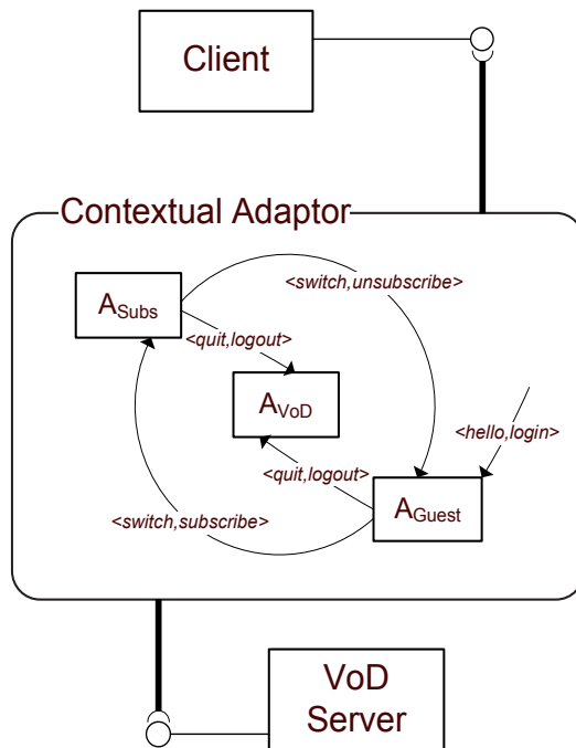
Fig. 2. VoD client/server interaction.
