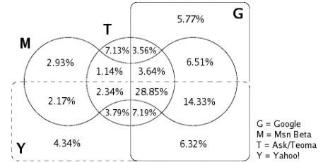
Figure 4: Results distribution across engines.
