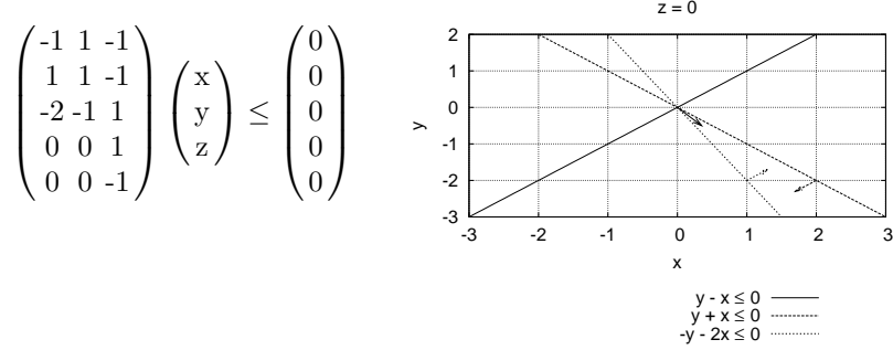
Fig. 1. LPCHECK procedure.
